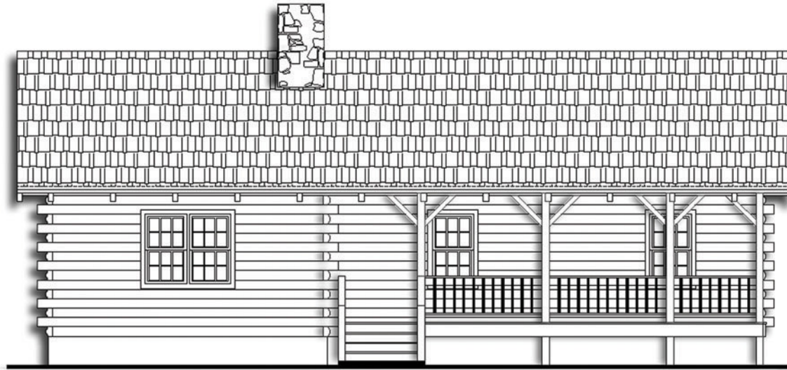
Front Elevation
